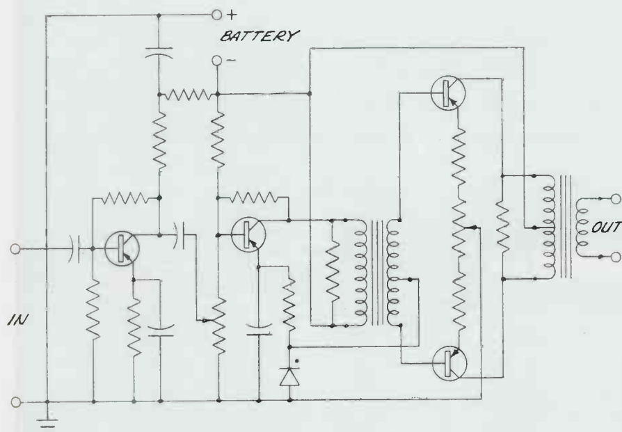
Figure 1. Line Amplifier.
